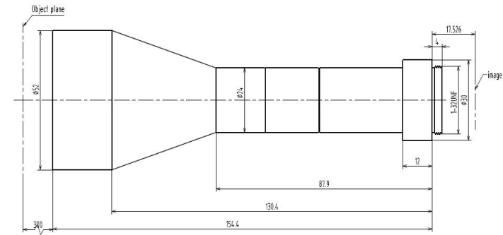
SNT23IR04W300C-I
