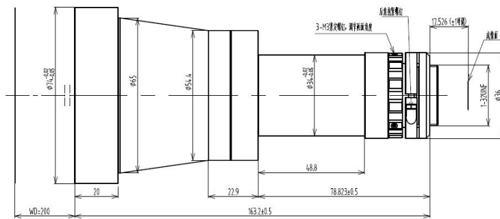
SNT23IR023W200C-I
