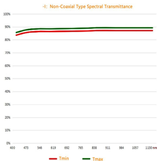
SNT23IR018W167C-I
