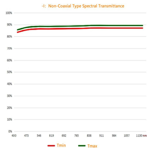
SNT23IR022W167C-I
