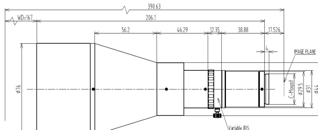
SNT23IR022W167C-I
